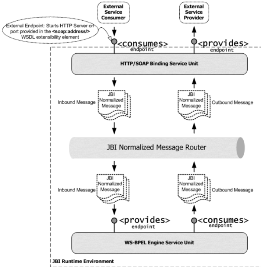
FIGURE 10 Routing Exchange Between the HTTP/SOAP Binding Component and the BPEL Service Engine
